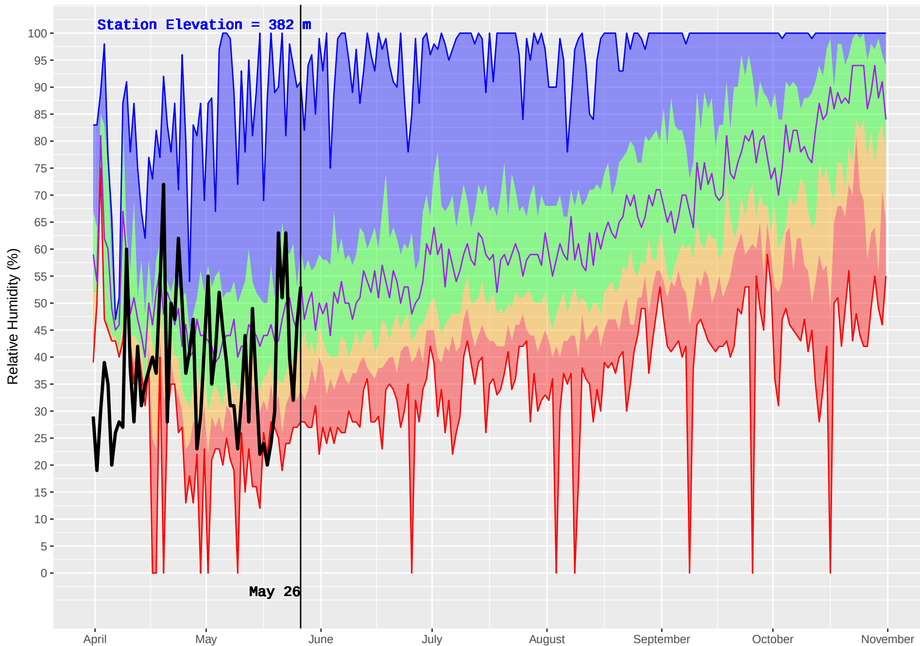
TELEGRAPH CREEK (110) : Historical (1978–2016) and Current (2018) Noon Relative Humidity
