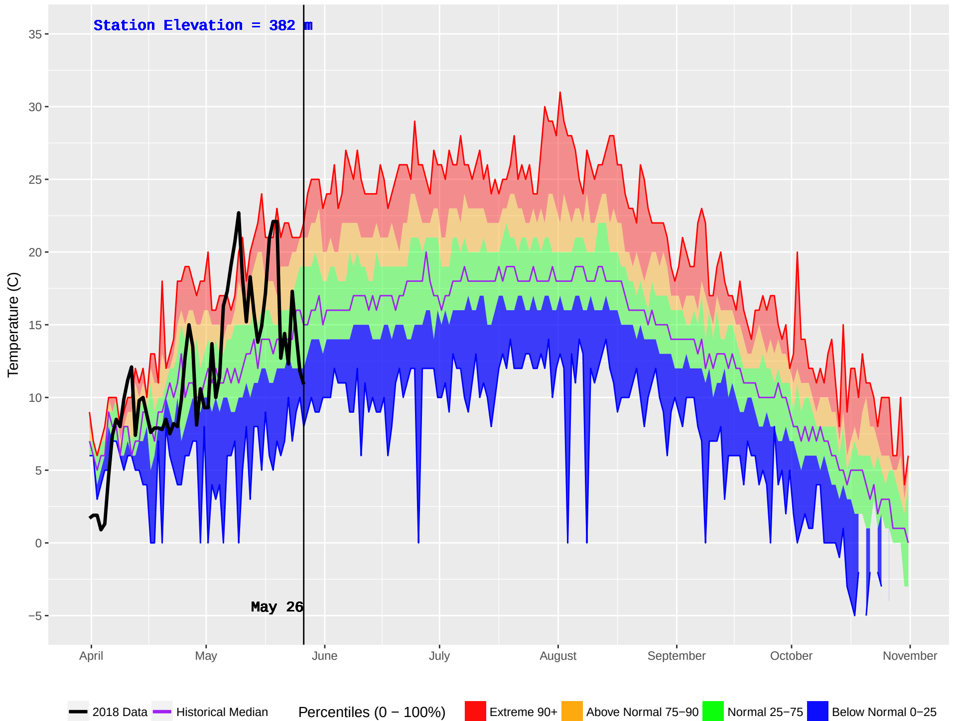
TELEGRAPH CREEK (110) : Historical (1978–2016) and Current (2018) Noon Temperature
